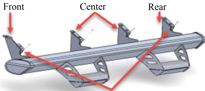
Outside bolt location closest to pinch weld.
