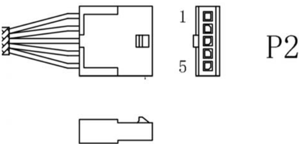
Female Molex 5-pin Connector P2 BLACK
