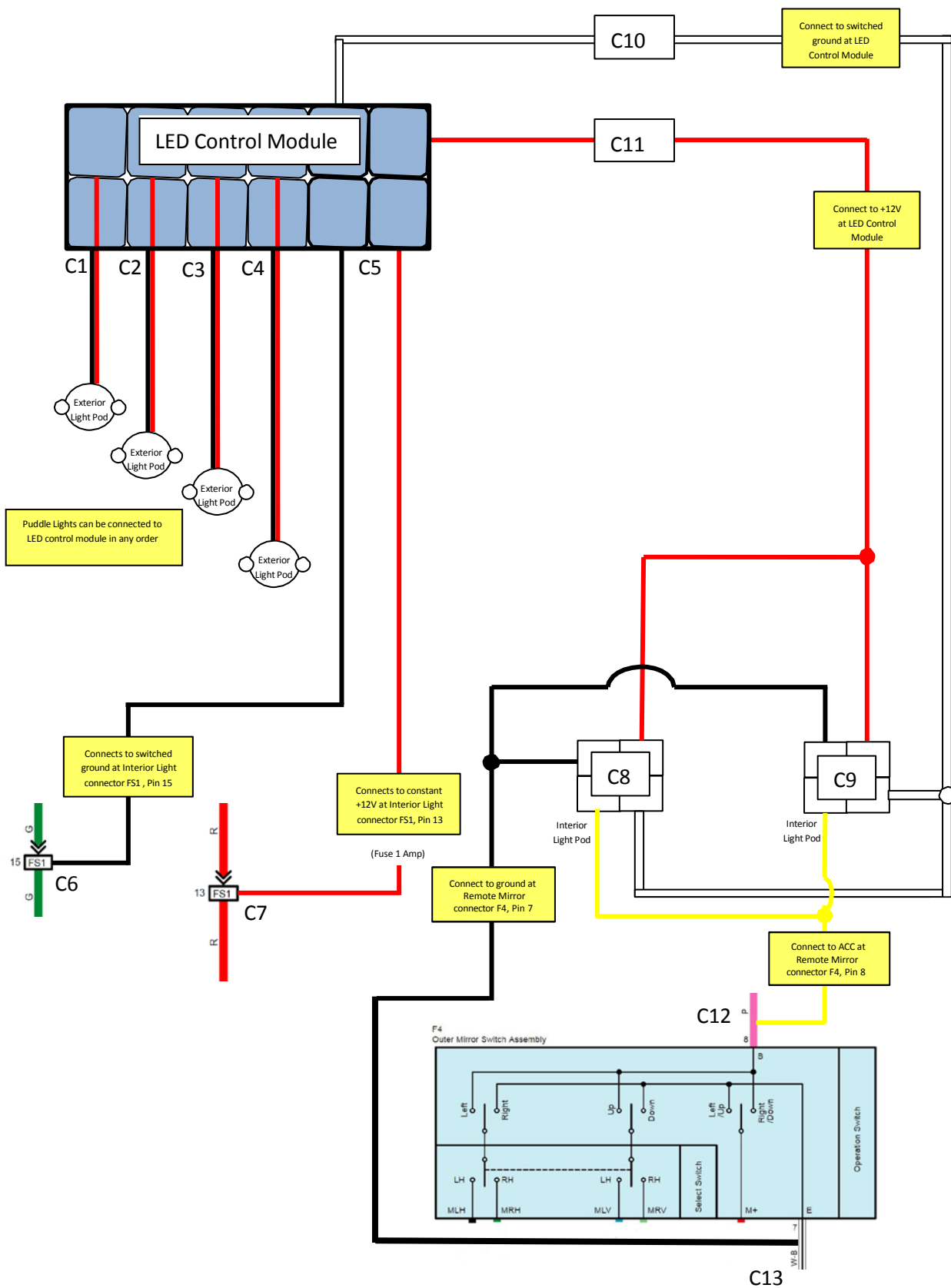
Block Diagram 4Runner Lighting Package
